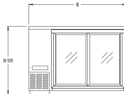
BBUC-50-SGD FRONT VIEW
