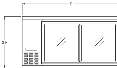
BBUC-69-SGD FRONT VIEW
