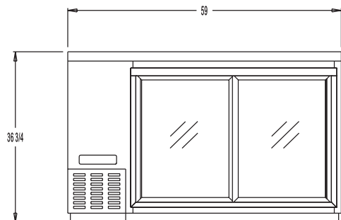
BBUC-59-SGD FRONT VIEW
