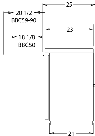
BBC50,59,69,79 & 90 SHALLOW SIDE VIEW
