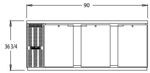
BBC90 FRONT VIEW
