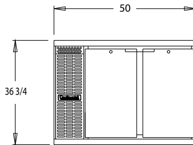
BBC50 FRONT VIEW
