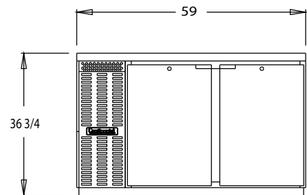
BBC59 FRONT VIEW
