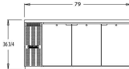
BBC79 FRONT VIEW
