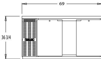
BBC69 FRONT VIEW
