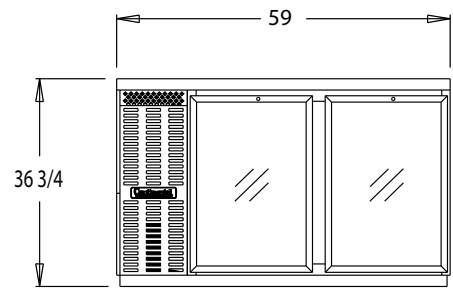
BBC59S-GD FRONT VIEW
