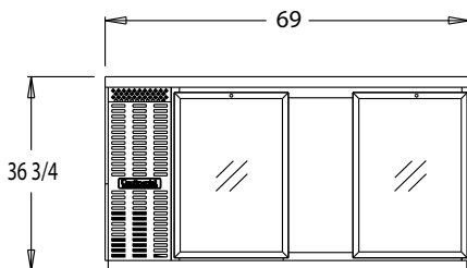
BBC69S-GD FRONT VIEW
