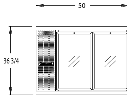
BBC50S-GD FRONT VIEW
