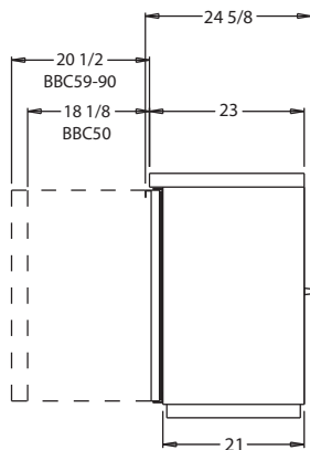
BBC50,59,69,79 & 90 SHALLOW SIDE VIEW
