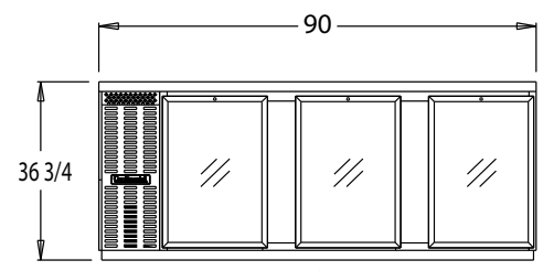
BBC90S-GD FRONT VIEW
