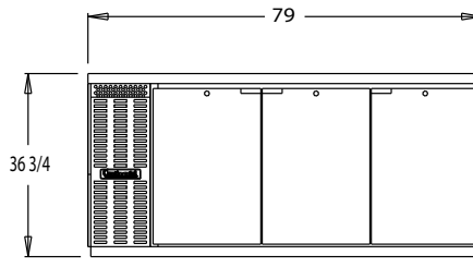
BBC79 FRONT VIEW
