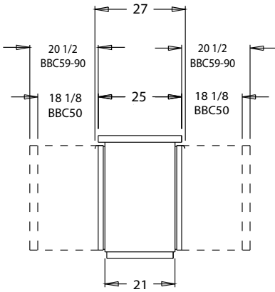
BBC50,59,69,79 & 90 SHALLOW SIDE VIEW
