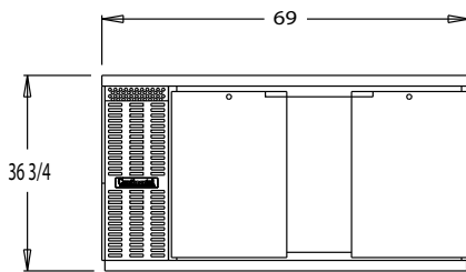
BBC69 FRONT VIEW
