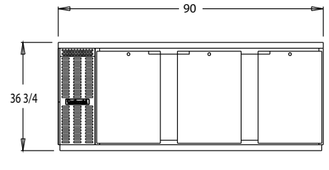
BBC90 FRONT VIEW
