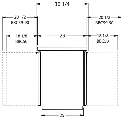
BBC50,59,69,79 & 90 SIDE VIEW
