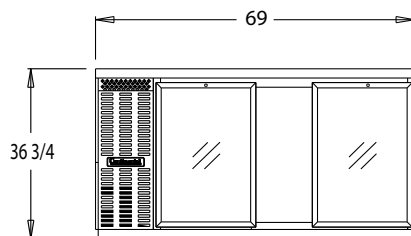
BBC69-GD FRONT VIEW
