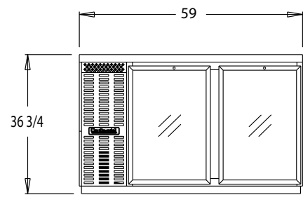
BBC59-GD FRONT VIEW
