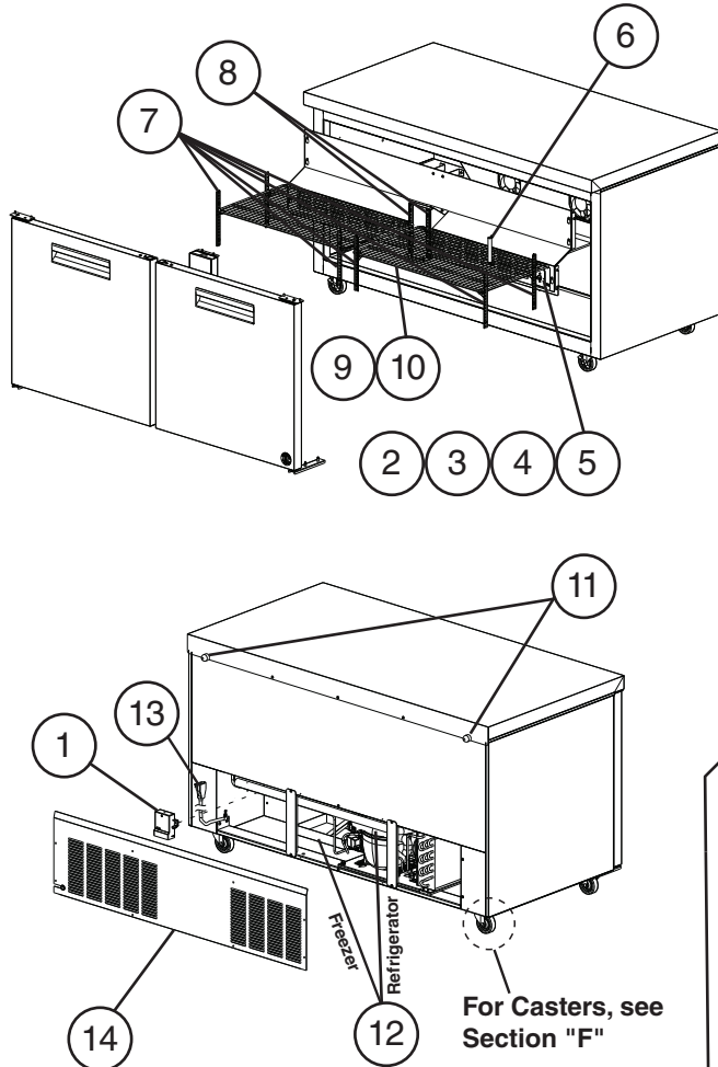
Model Shown: CRMF60
