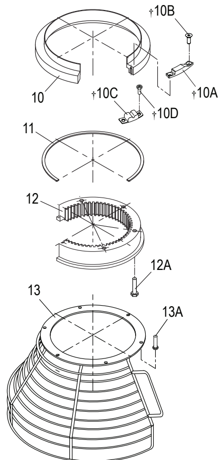
Fixed Bowl Guard before S/N 7610884 or S/N 7650835
