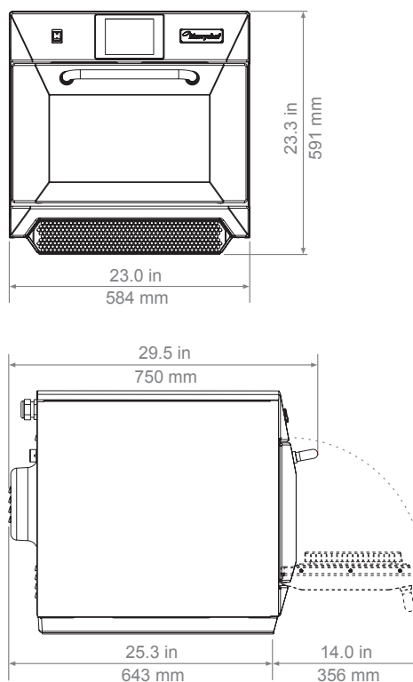
Oven Dimensions
