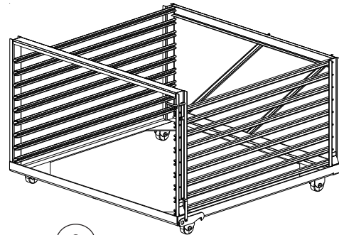
11207 Roll-In Pan Rack- DFG100
