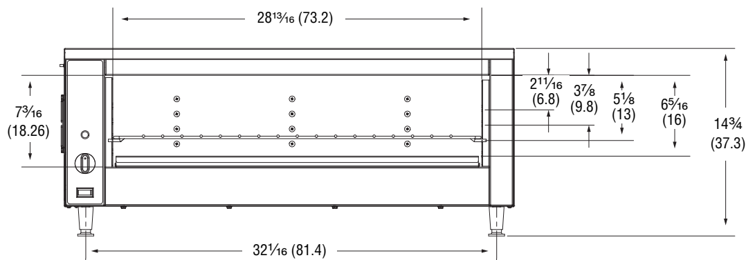
Front View
