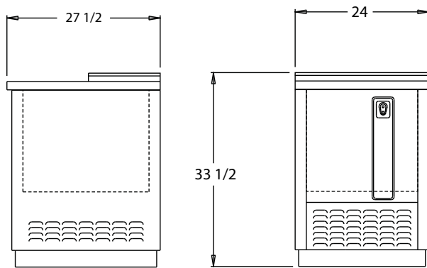
CBC24 FRONT VIEW
