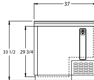
CBC37 FRONT VIEW
