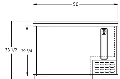
CBC50 FRONT VIEW
