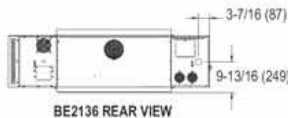
BE2136 REAR VIEW
