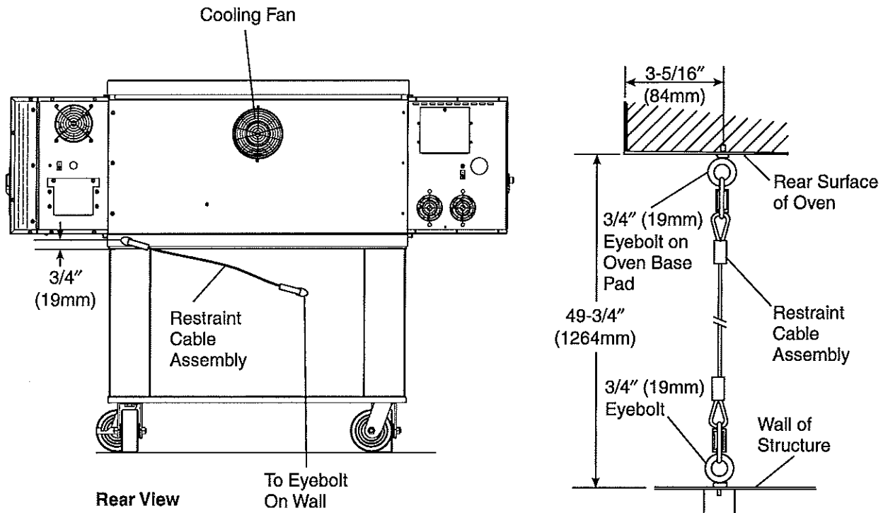
Figure 2-8. Restraint Cable Assembly Installation
