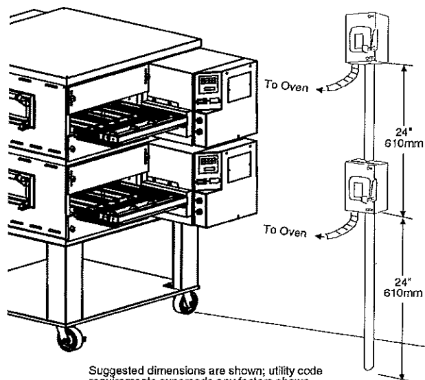
Figure 2-9. Typical BE2136-Series Oven(s) Installation
