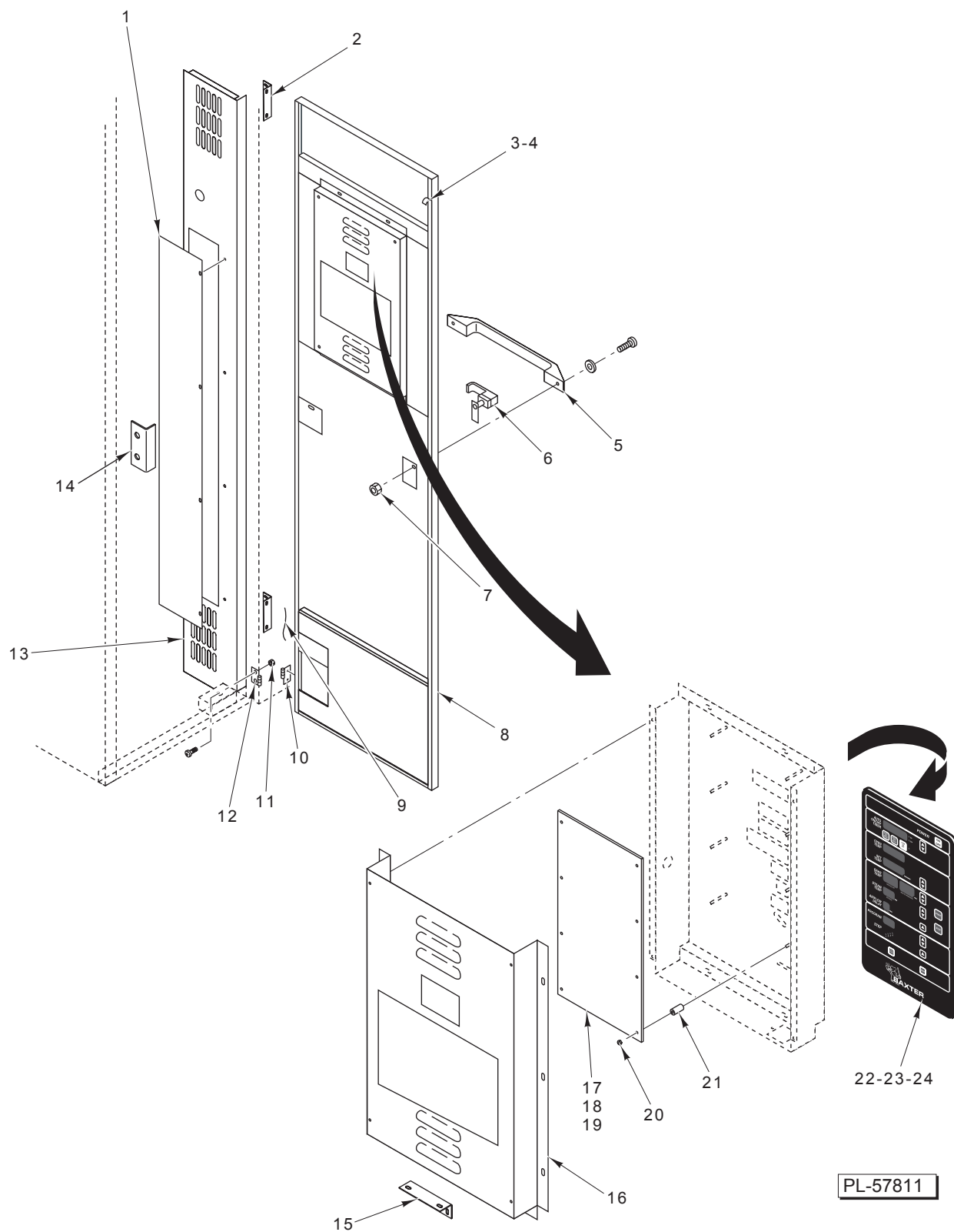
CONTROL CABINET, DOOR, AND CONTROLLER (ML-132359)
