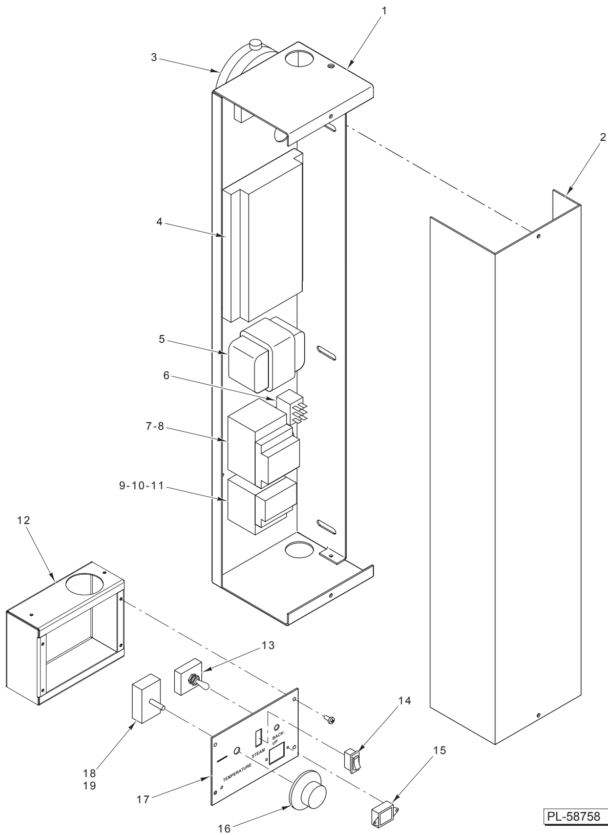
COMPONENT BOX (ML-132359)
