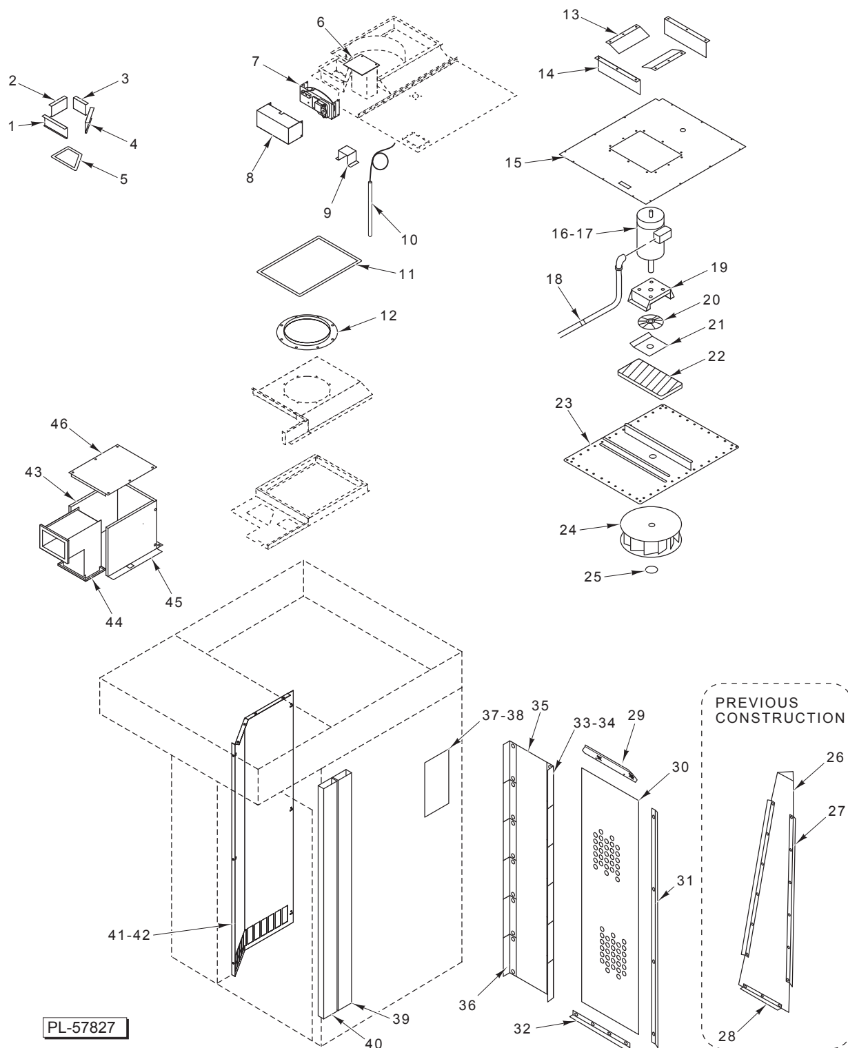
BLOWER, PANELS, AND VENTS (ML-132281)
