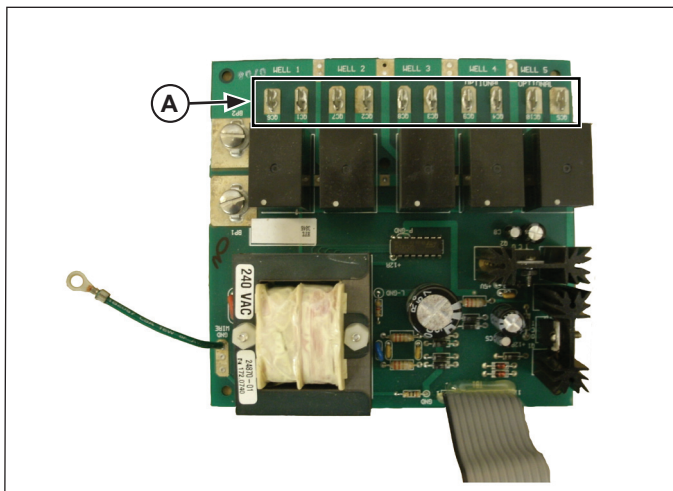
Figure 1. Old Relay Board
