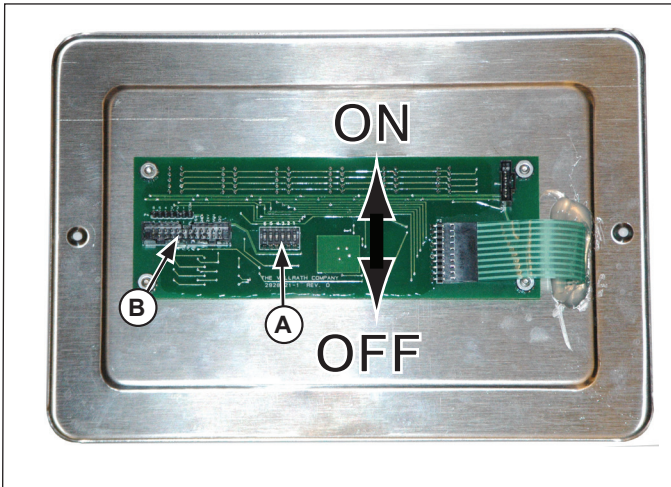
Figure 3. Logic Board
