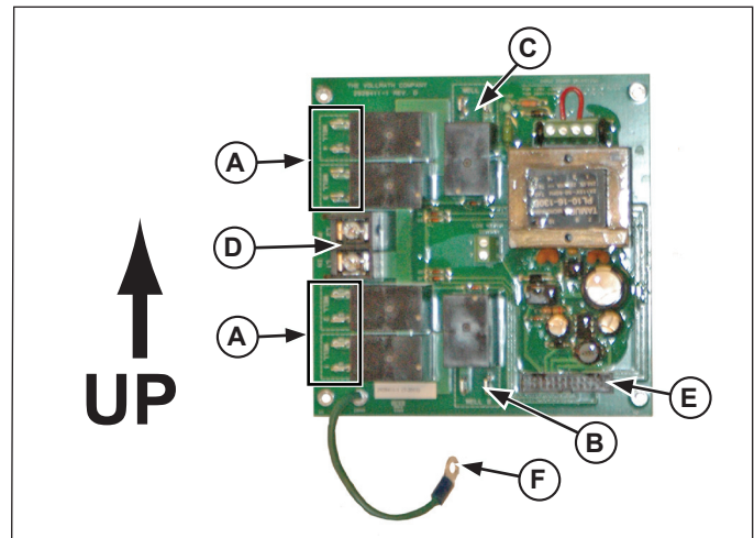
Figure 2. New Relay Board
