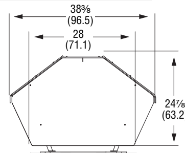
Classic Economy Buffet NSF
