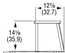
Single Shelf Cafeteria Standard
