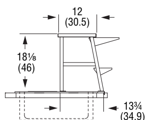
Double Shelf Cafeteria Standard
