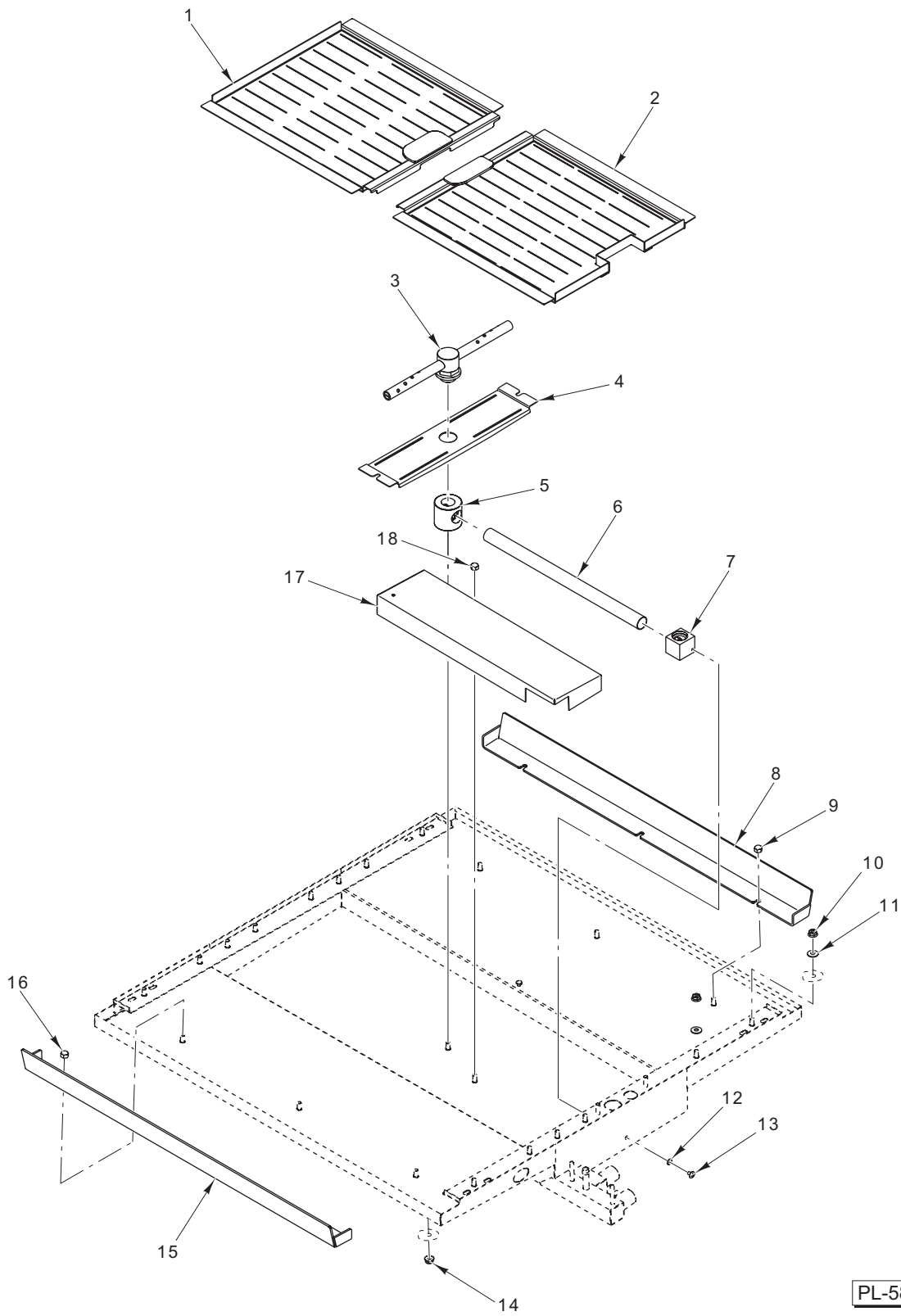
DRAIN TRAY
