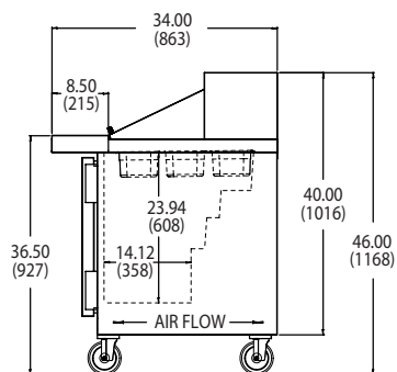
VUR-6-24 BT, VUR-6-30 BT SIDE VIEW
