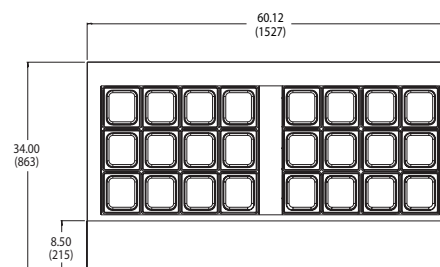
VUR-5-24BT TOP VIEW
