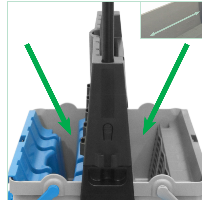
Fill scrub board bucket with water to the fill line then place bucket on carriage. Fill StayClean bucket with water and cleaning agent to fill line, place on carriage.
