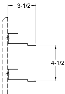
DETAIL OF PAN SLIDE
