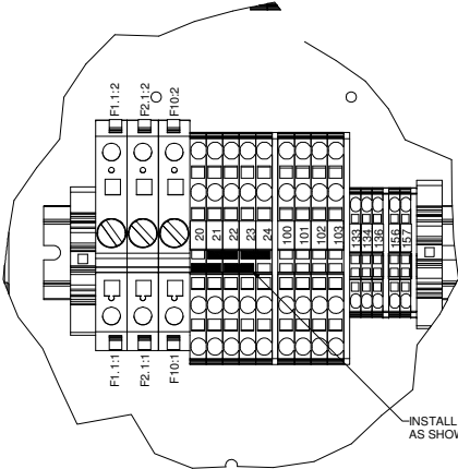
DETAIL A INSTALL JUMPERS AS SHOWN
