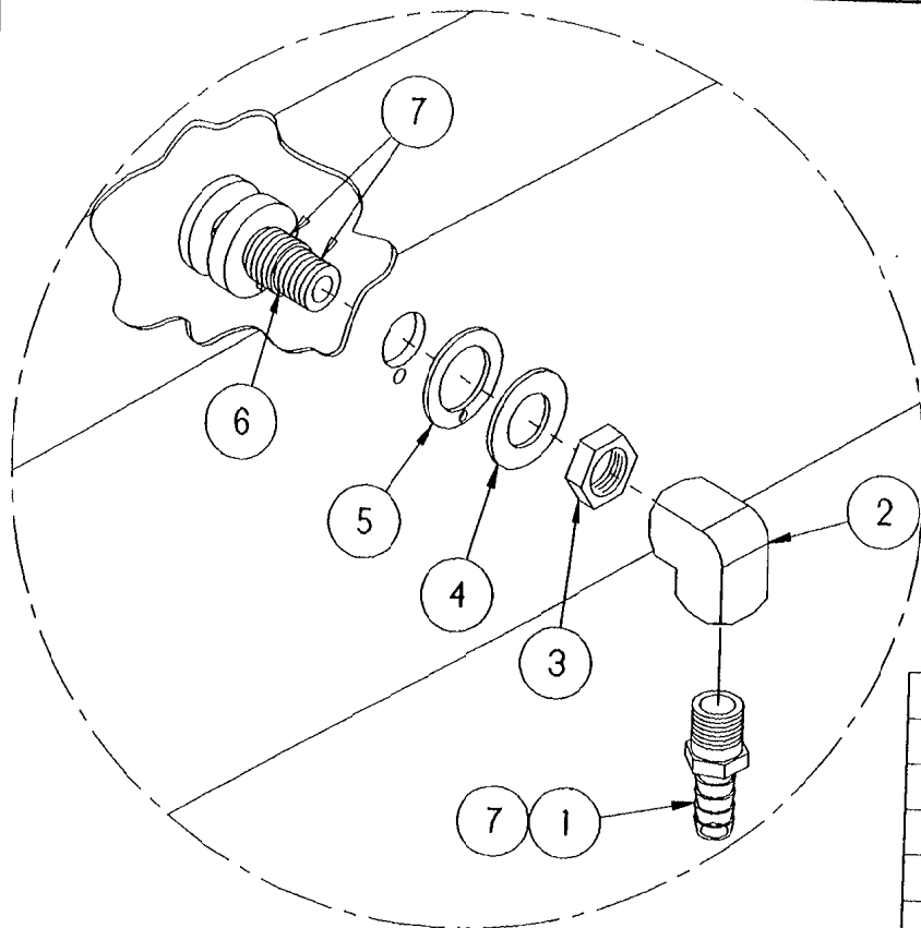
TYPICAL APPLICATION
