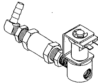
ASSEMBLED UNIT
