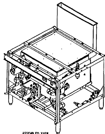
ASSEMBLED VIEW
