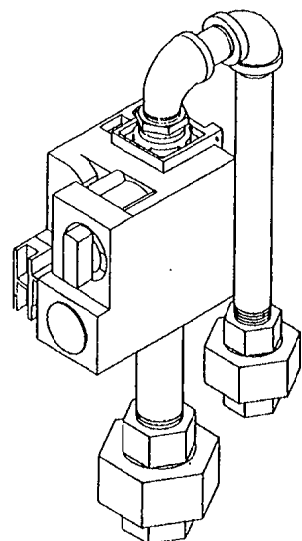
ASSEMBLED VIEW
