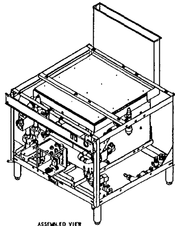
ASSEMBLED VIEW
