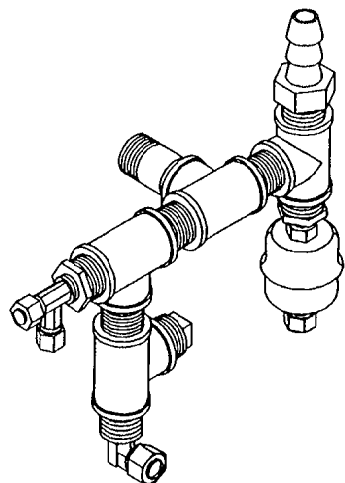
ASSEMBLED VIEW
