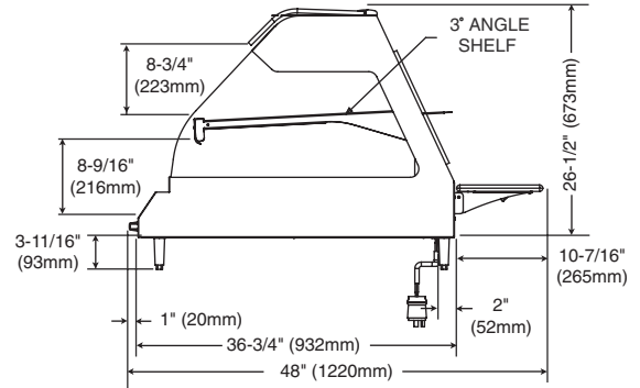
ED2-2S PROFILE
