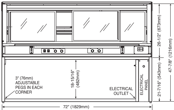
ED2SYS-72/2S
