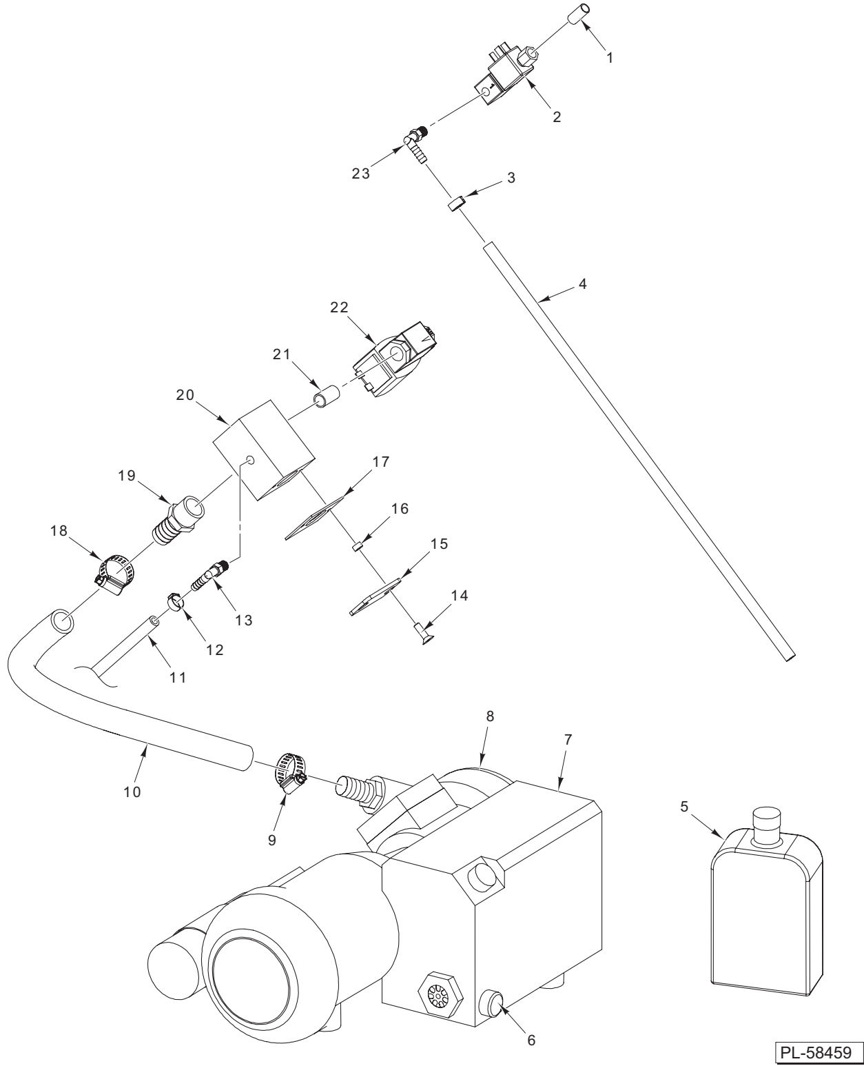
VACUUM PUMP
